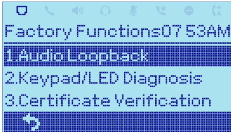
Figure 19: Factory Functions
